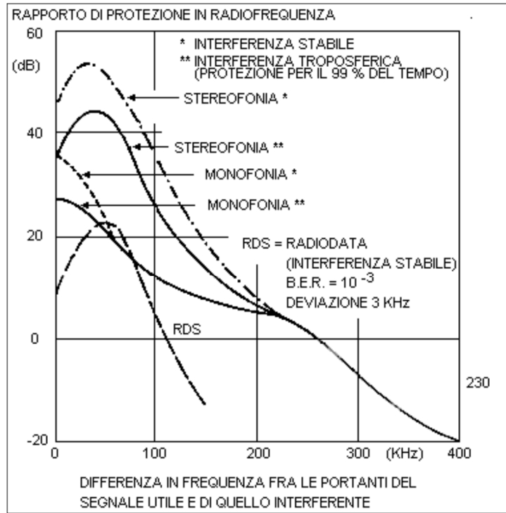
Figure 4 Protection ratios for FM radiophony (max. deviation: ± 75 KHz) Fig.5 shows the protection ratio curves for the three services.
